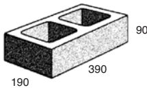
20.71 Half high
